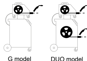
G model
